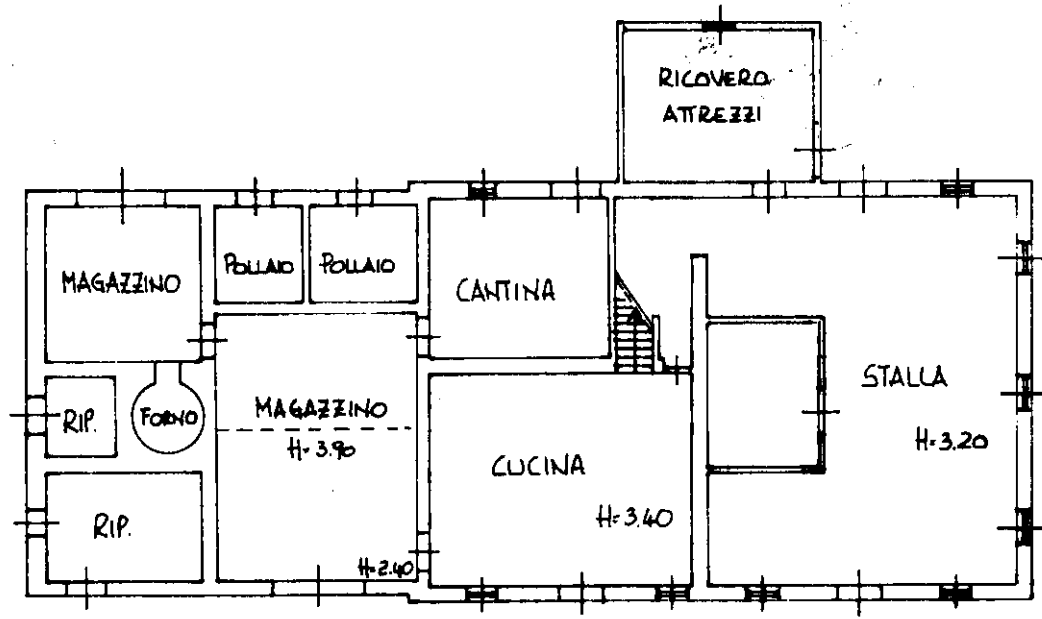
PIANO TERRA
